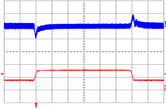
Fig. 1.2V.11: Output voltage response to load current step-change (3.75 A – 7.5 A – 3.75 A) at V_{in} = 48 V. Top trace: output voltage (100 mV/div.). Bottom trace: load current (5 A/div.). Current slew rate: 0.1 A/ \mu s. C_o = 1 \mu F ceramic. Time scale: 0.2 ms/div.
