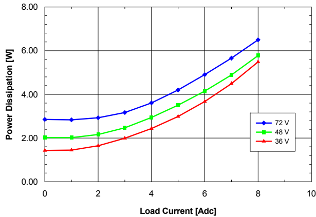
Fig. 6.0V.7: Power dissipation vs. load current and input voltage for SQ48T/S08060 converter mounted vertically with air flowing from pin 3 to pin 1 at a rate of 300 LFM (1.5 m/s) and T_a = 25\text{ }^\circ\text{C} .
